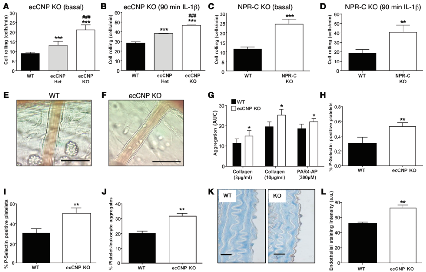
Figure 3. Leukocyte and platelet hyperreactivity in ecCNP KO mice. Basal and IL-1 \beta -stimulated (5 ng/mouse; i.p.) leukocyte rolling was significantly greater in ecCNP KO ( A and B ) and NPR-C KO ( C and D ) mice compared with WT littermates. Representative images of basal rolling are shown ( E and F ). Platelet aggregation in response to collagen (3 \mu g/ml and 10 \mu g/ml) and PAR4-AP (300 \mu M; G ), basal and PAR4-AP-triggered platelet expression of P-selectin ( H and I ), and the level of circulating platelet-leukocyte aggregates ( J ) was greater in ecCNP KO mice compared with WT littermates, implying that CNP regulates platelet function (and leukocyte recruitment) via inhibition of P-selectin expression. Endothelial P-selectin expression was also significantly greater in the aorta of ecCNP KO versus WT mice ( K and L ). Data are represented as the mean \pm SEM. n = 10 for leukocyte studies; n = 6 for platelet reactivity and flow cytometry experiments. * P < 0.05 , ** P < 0.01 , *** P < 0.001 , significantly different from WT littermates; ### P < 0.001 , significantly different from heterozygote littermates. Scale bars: 50 \mu m ( E and F ); 20 \mu m ( K ).
